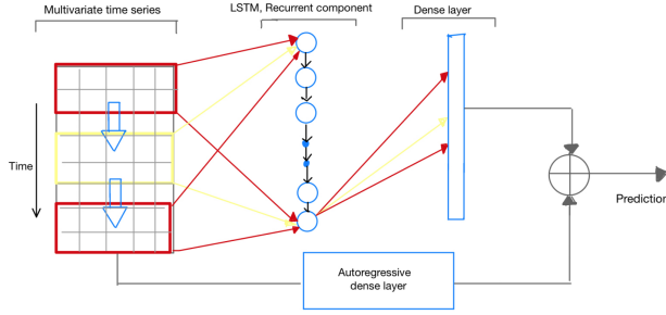
Figure 5: TVP-VARNet
